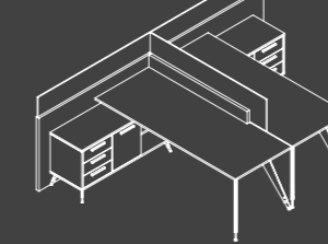
2'Lİ ÇALIŞMA MASASI WORKSTATION FOR 2 PERSONS PNLYWS PNL160WS GZAKS01 - Metal Kalemlik - Metal Pencil Box GPNLWS - Ahşap Duvar Bölme - Panel Wooden Wall Partitional Panel
