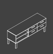
4 ÇEKMECELİ RAFLI ETAJER 4 DRAWERS WITH OPEN SHELVES 170X50X65 cm ENG170ESTD
